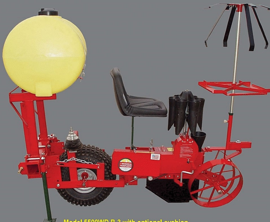
Model 5500WD B-3 with optional cushion seat and 5600 carousel tray holder
